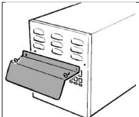
Figure 16 Weather Shield Installation
