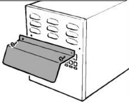
Figure 37 Weather Shield Fixings
