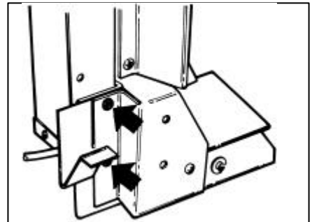
Figure 31 Electrical control unit fixings
