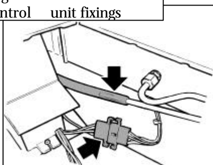
Figure 11 Fan loom & vacuum pipe connections
