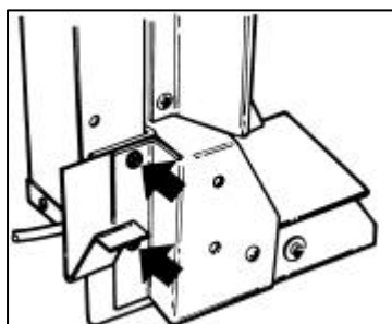
Figure 10 Electrical control unit fixings
